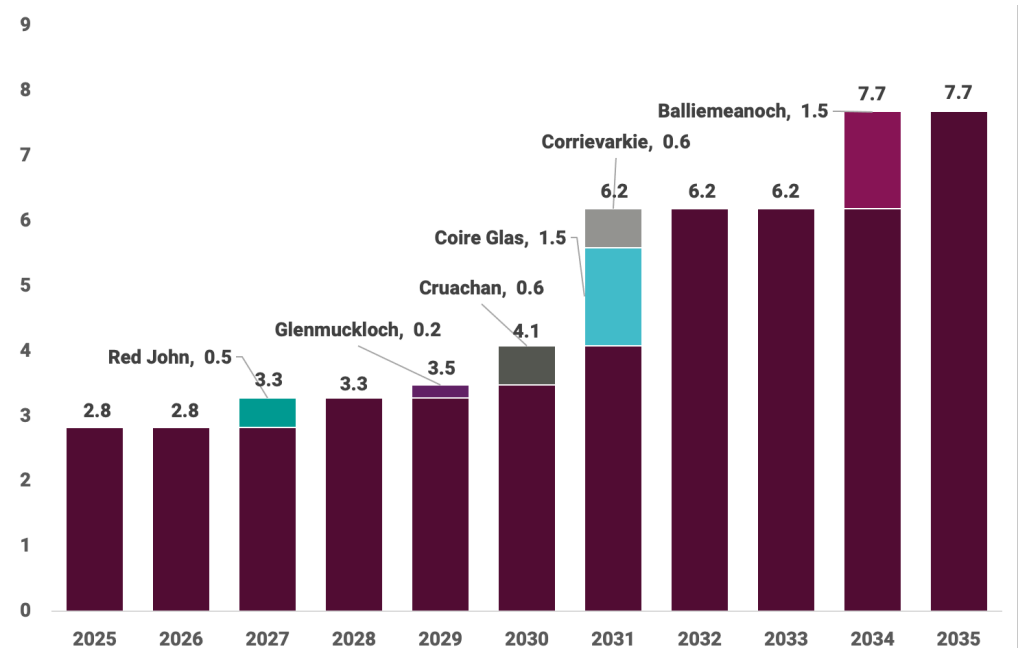
Figure 4.2: UK Installed Output Capacity over Time (GW), 2025-2035
