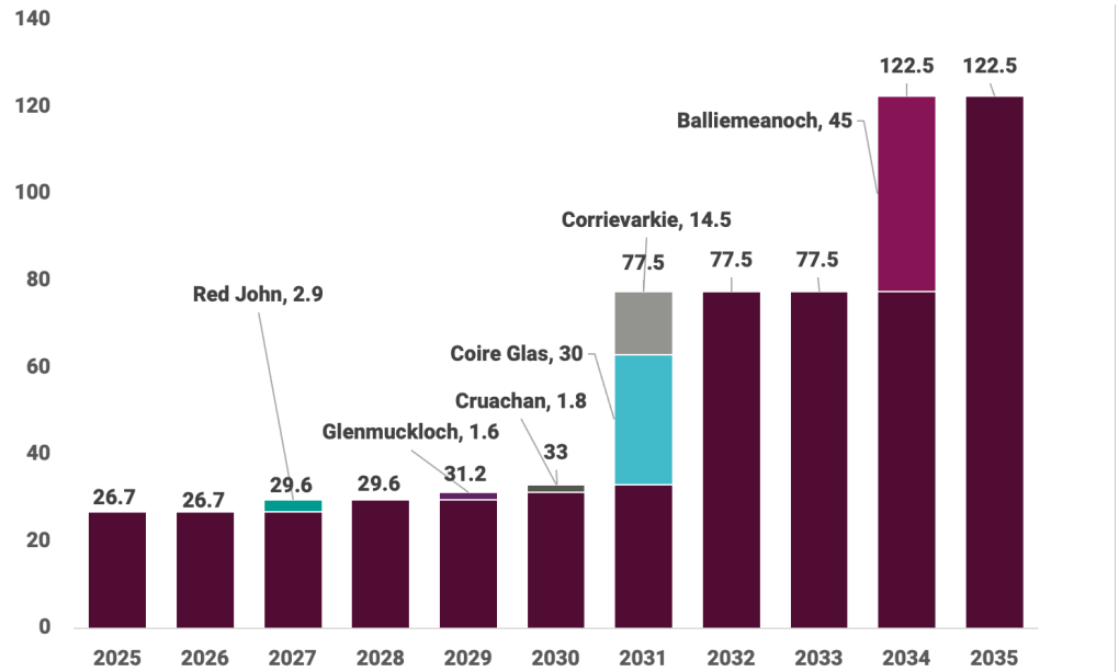
Figure 4.1: UK Installed Pumped Storage Hydro Capacity over Time (GWh), 2025-2035
